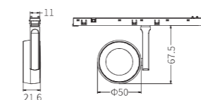
Track Coin - D50
