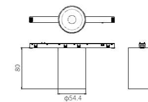
Cylinder Downlight R Lens - D54
