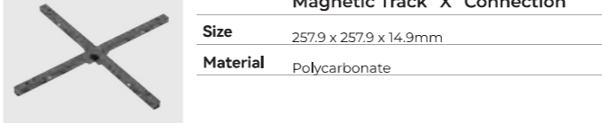
Magnetic Track "X" Connection
