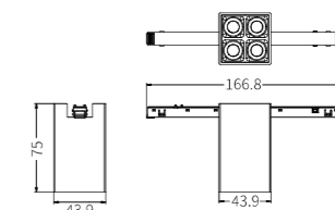
Cylinder Downlight SQ Cell Integrated - D44
