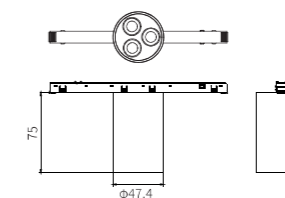
Cylinder Downlight Cell - D47
