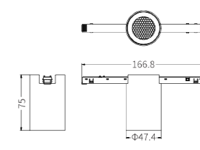
Cylinder Downlight R Lens Integrated - D44
