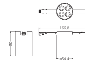
Cylinder Downlight R Cell - D54
