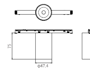
Cylinder Downlight R Lens - D44
