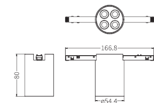
Cylinder Downlight R Cell Integrated - D54
