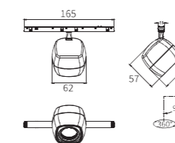
Track CoinSQ - D62
