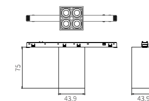
Cylinder Downlight SQ Cell - D44
