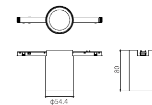
Cylinder Downlight R Lens Integrated - D54
